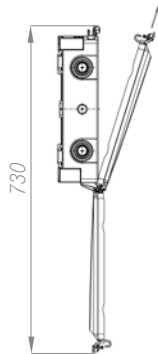
Opening of cover, cover can be removed at angle of 30°
