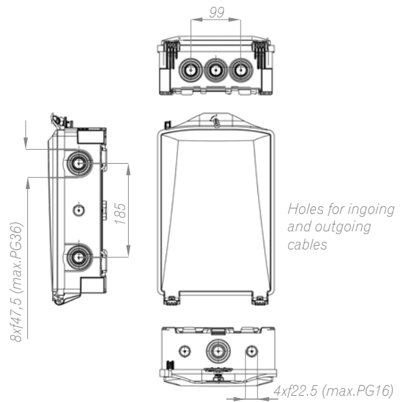
ZK cable service box equipped with 3-pole or 4-pole fuse base PBD 00
