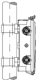
Mounting on electric traction pole
